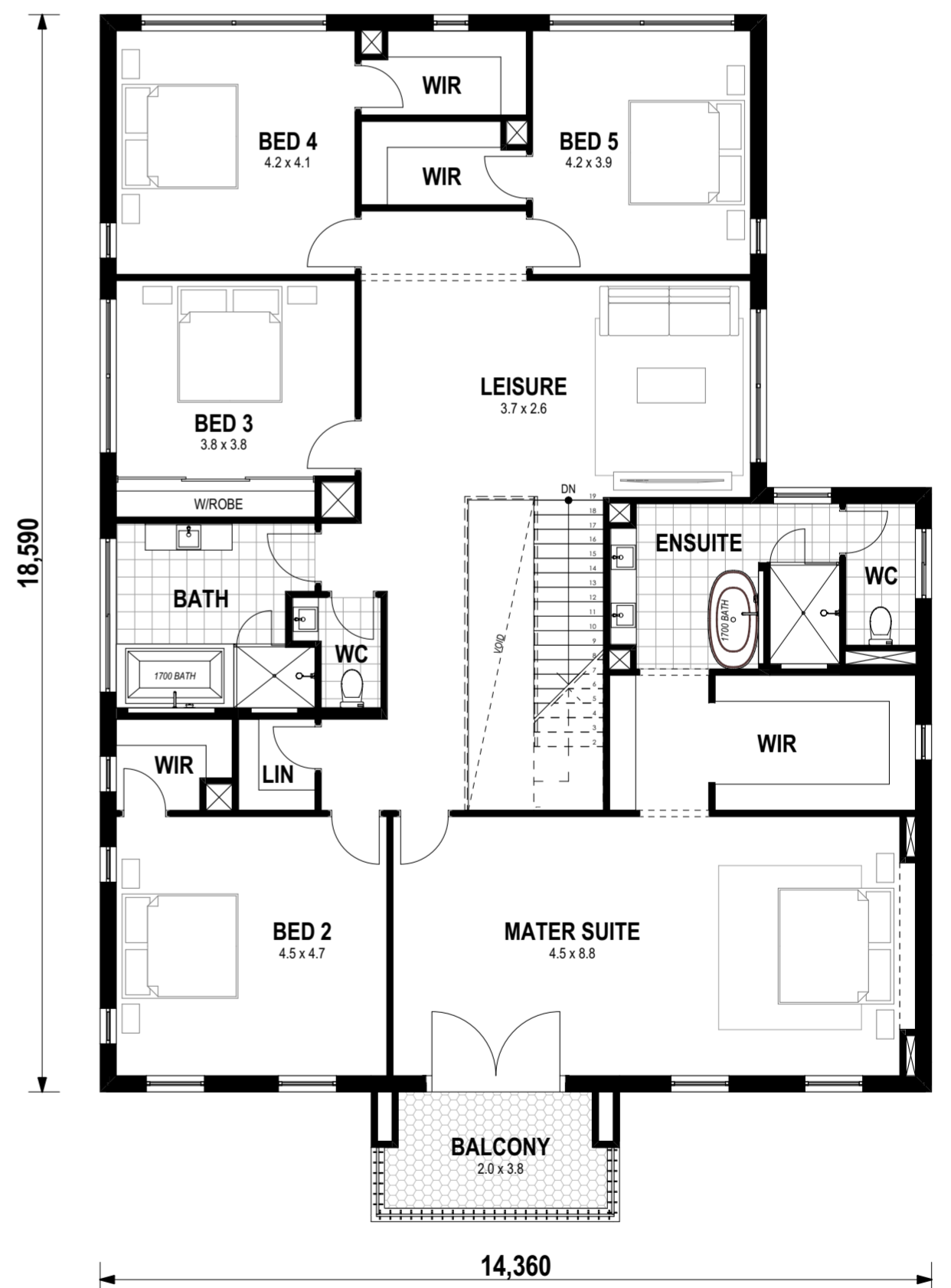
○ FIRST FLOOR 1:100
